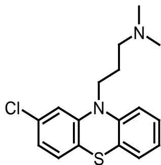
Chlorpromazine
