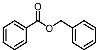
Benzyl benzoate
